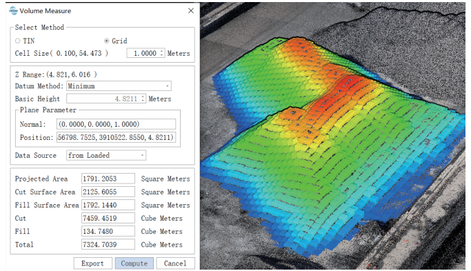
Volume Measurement
